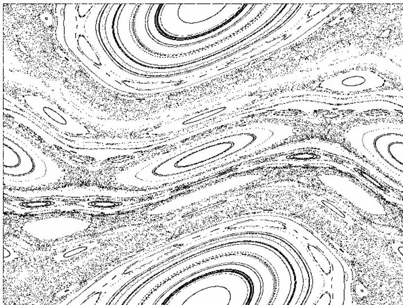
Figure 3: The change of a certain parameter converts, even in classical mechanics, „regular“ into „chaotic“ motion. All dots belong to one trajectory!
